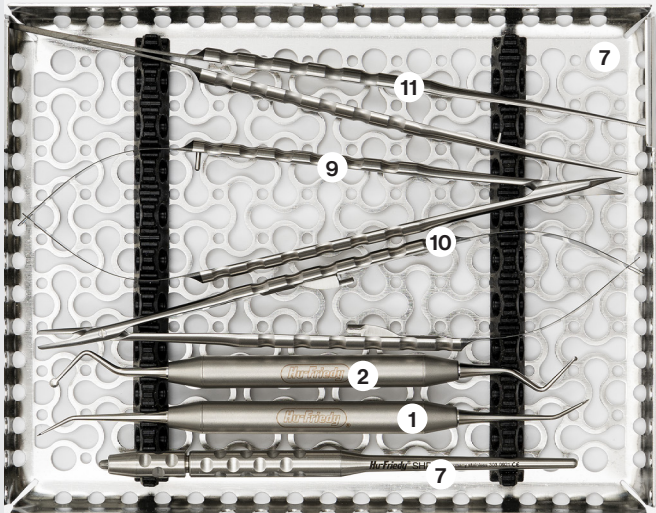
IME12DIN1_ IMS™ Infinity Series™ 1/2 DIN Cassette with accessory area - 10 Instrument Dimensions: 152 x 184 x 34 mm
